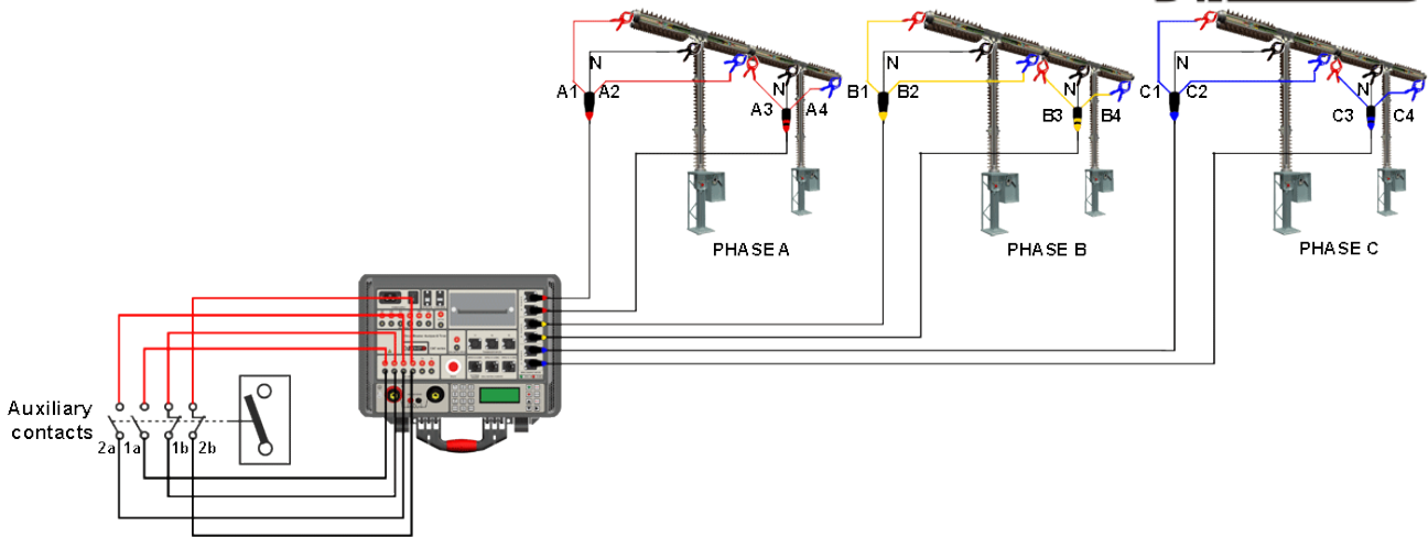
Connecting the main contact timing cables and auxiliary timing cables to a test object
