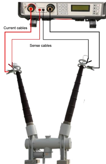
Micro Ohmmeter cable connection on a dead tank circuit breaker
