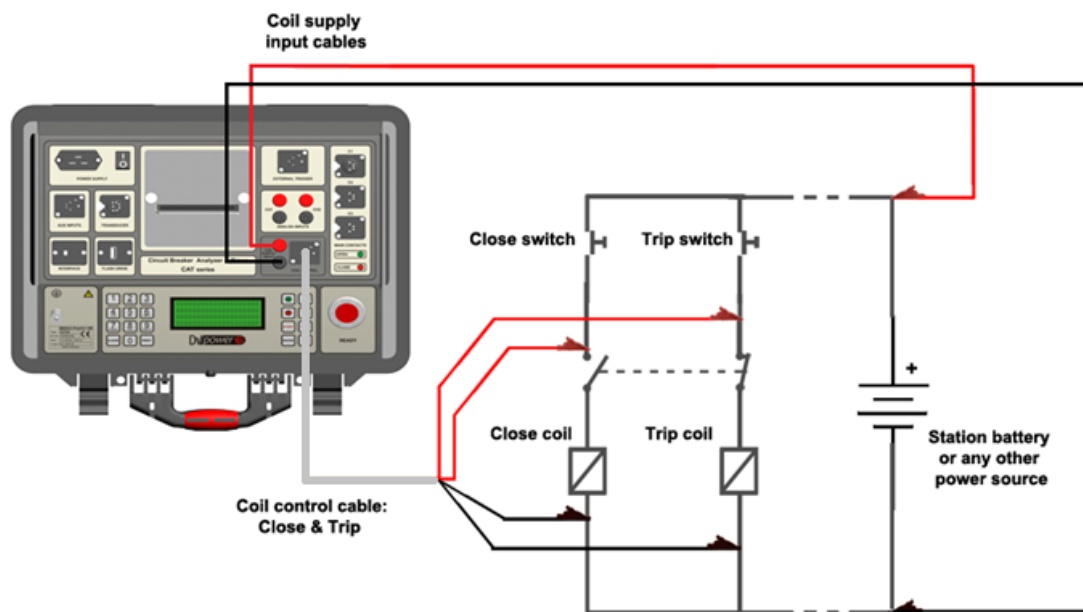
Connecting the coil control cables to circuit breaker control circuit
