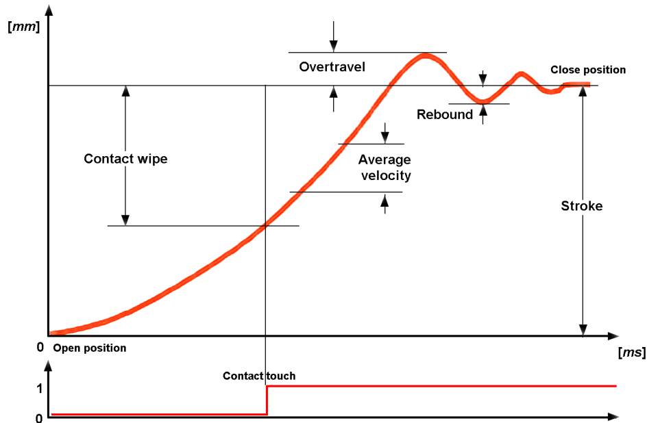
Travel curve and important travel parameters
