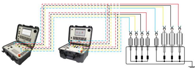
Connecting TWA500 and TRT500 to a three-phase transformer
