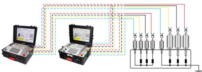
Connecting TWA400 and TRT400 to a three three-phase transformer
